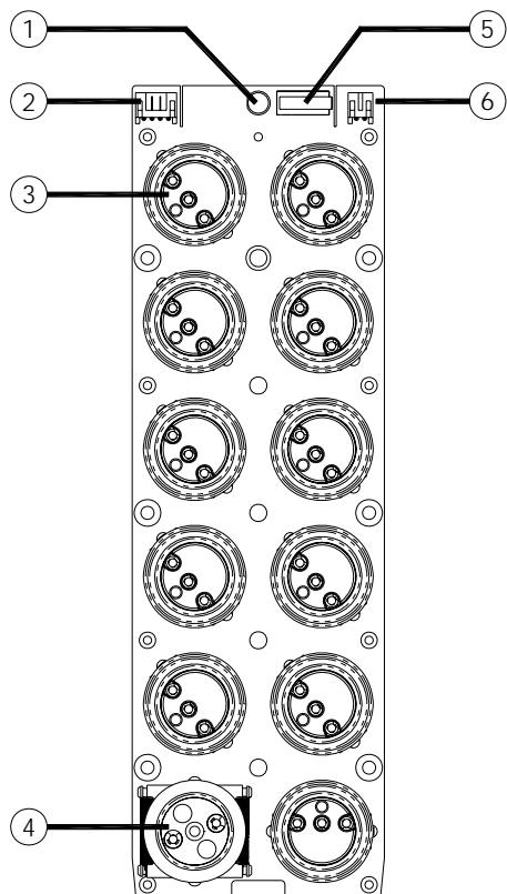
(PCB Front View)
