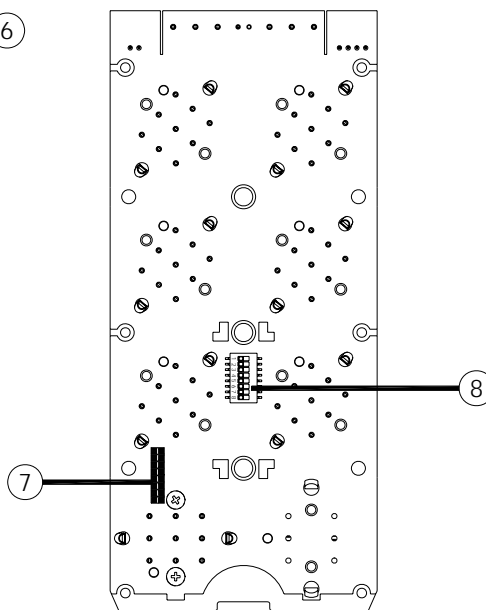
(PCB Back View)
