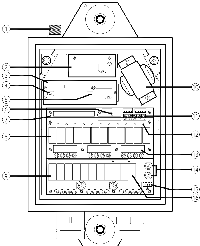
(Alpha 3000D2 & D3 Models Receiver Internal View)
