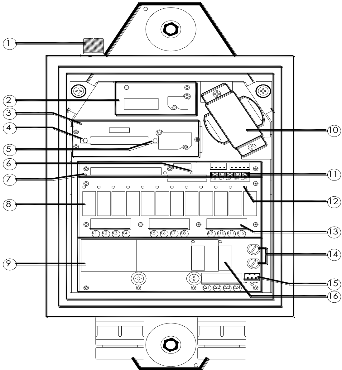
(Alpha 3000F2 & F3 Models Receiver Internal View)
